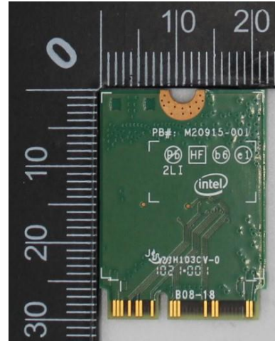
Adaptor back
