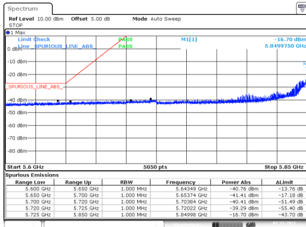
BE-NR-LOW, SISO-B, 802.11a20-6Mbps, Ch173
