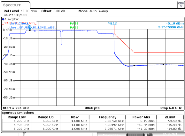
BE-NR-HIGH, MIMO-B, 802.11ax160-HE0, Ch163
