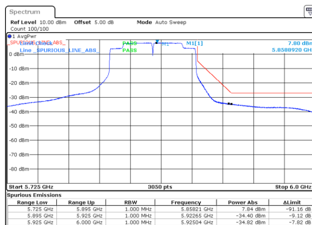
BE-NR-HIGH, SISO-B, 802.11ac80-VHT0, Ch171
