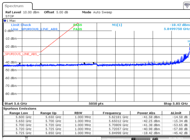
BE-NR-LOW, MIMO-A, 802.11n20-HT8, Ch173
