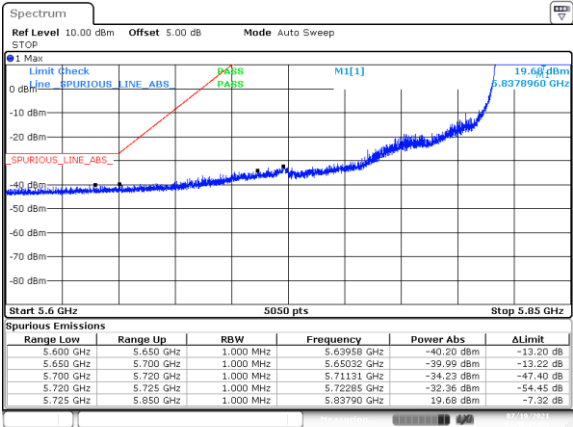
BE-NR-LOW, MIMO-A, 802.11n40-HT8, Ch167
