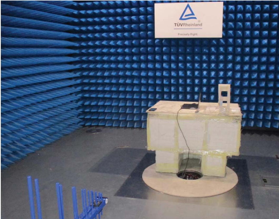
Photo 1 Photograph test setup radiated emissions 30-1000 MHz
