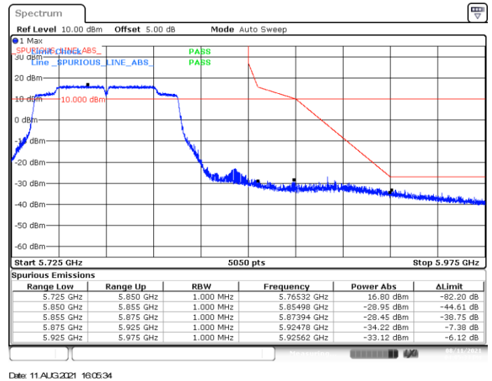
BE-NR-HIGH, SISO-B, 802.11ac80-VHT0, Ch155
