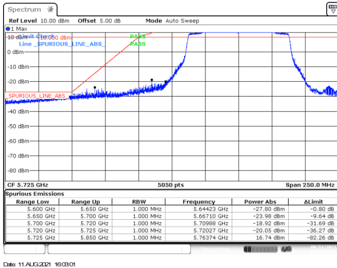
BE-NR-LOW, SISO-B, 802.11ac80-VHT0, Ch155
