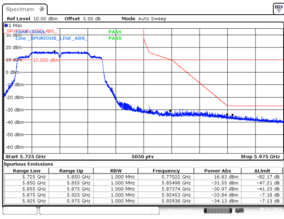
BE-NR-HIGH, MIMO-B, 802.11ac80-VHT0, Ch155
