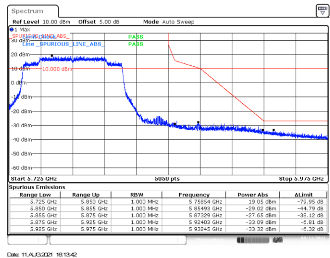
BE-NR-HIGH, SISO-B, 802.11ax80-HE0, Ch155
