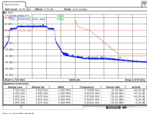
BE-NR-HIGH, MIMO-B, 802.11ax80-HE0, Ch155
