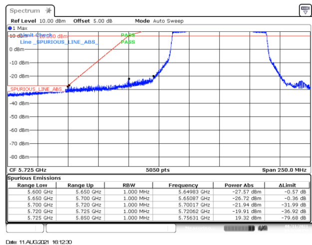
BE-NR-LOW, SISO-B, 802.11ax80-HE0, Ch155
