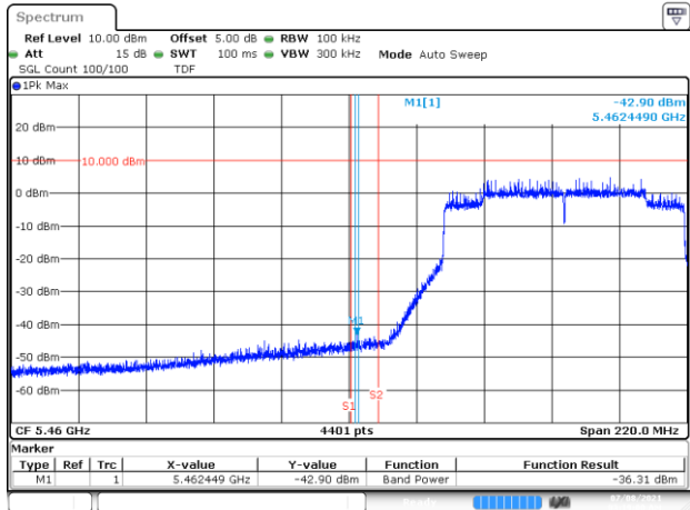
BE-NR-LOW, MIMO-A, 802.11ax80-HE0, Ch106
