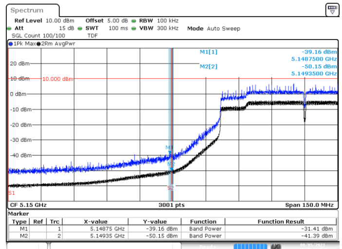
BE-R-LOW, SISO-A, 802.11ac80-VHT0, Ch42
