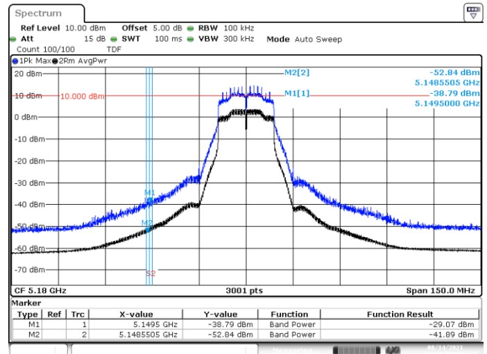
BE-R-LOW, SISO-A, 802.11n20-HT0, Ch36
