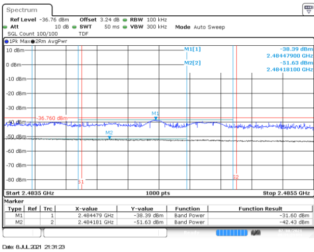
BE-R-HIGH-2MHz, SISO-B, 802.11ax40-HE0, Ch12
