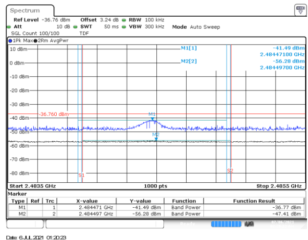
BE-R-HIGH-2MHz, MIMO-A, 802.11ax40-HE0, Ch9
