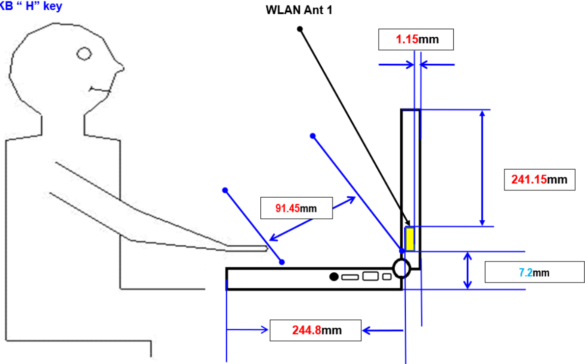
*Distance between the transmit antennas and the user 天線到KB “H” key
