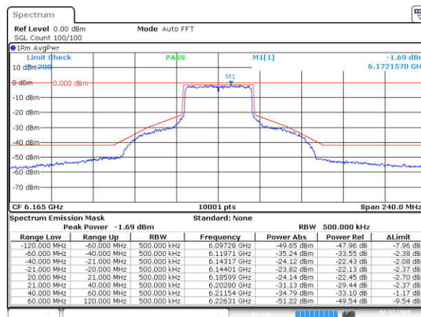
SISO A-802.11ax-40MHz-Ch43-6165MHz-MCS0
