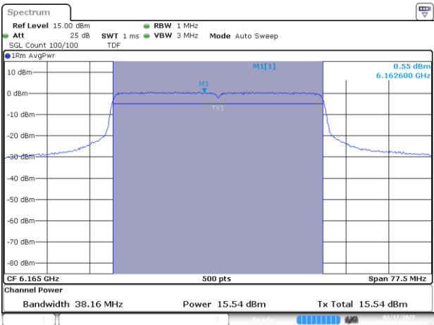
SISO A-802.11ax-40MHz-Ch43-6165MHz-MCS0
