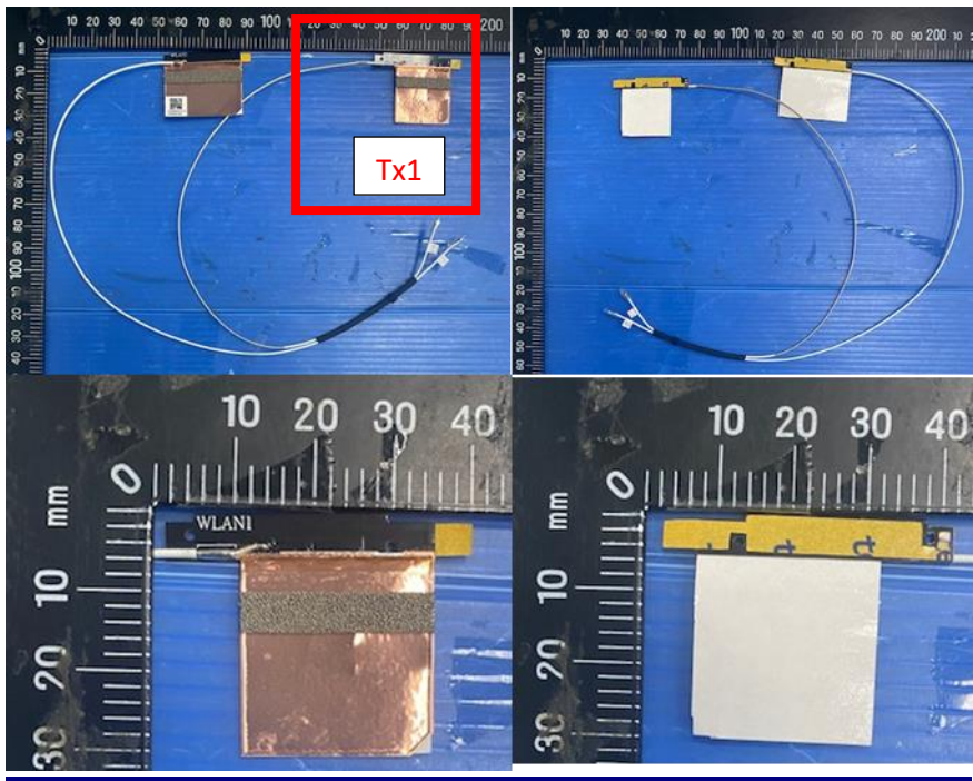
Ant 1 (Tx1) Antenna Photo
