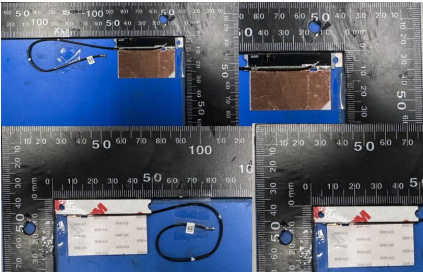
Main Antenna Photo (Front/Back):
