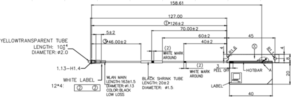
Main Antenna Drawing:
