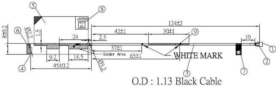
Tx1 Antenna Dimensioned Drawing:
