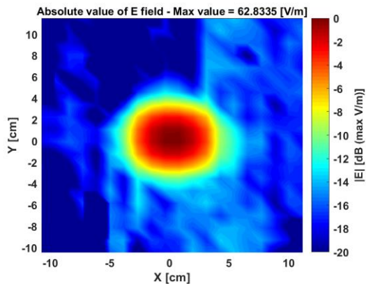
Field variation through the maximum along the E-field polarization
