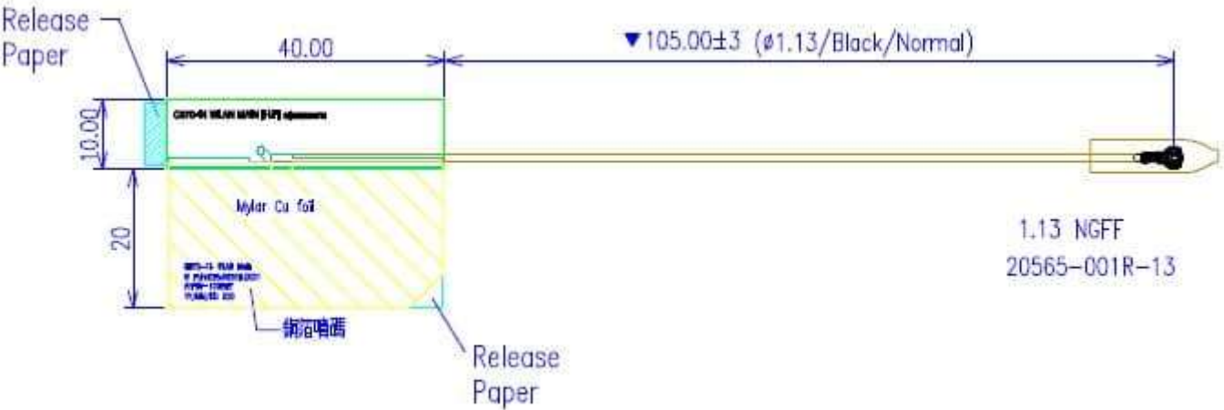
Main Antenna Dimensioned Drawing:
