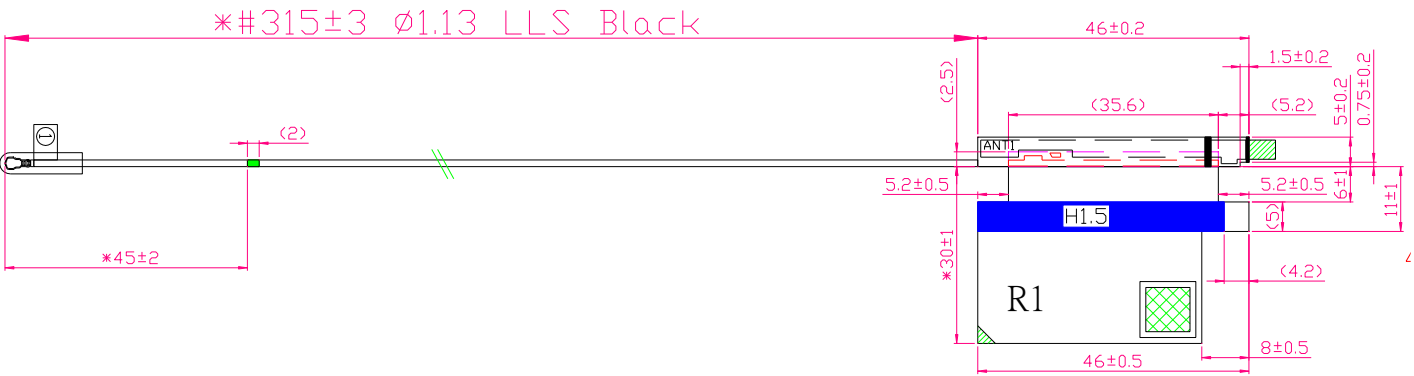
Tx1 Antenna Dimensioned Drawing:
