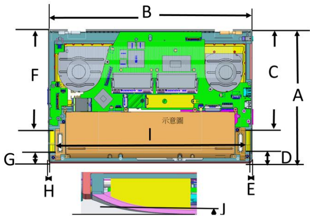
Antenna Host Platform location #1
