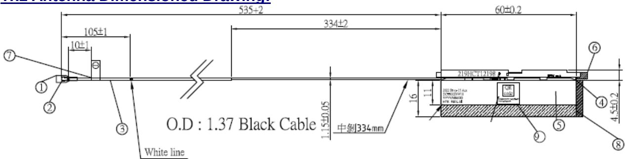
Tx1 Antenna Dimensioned Drawing:
