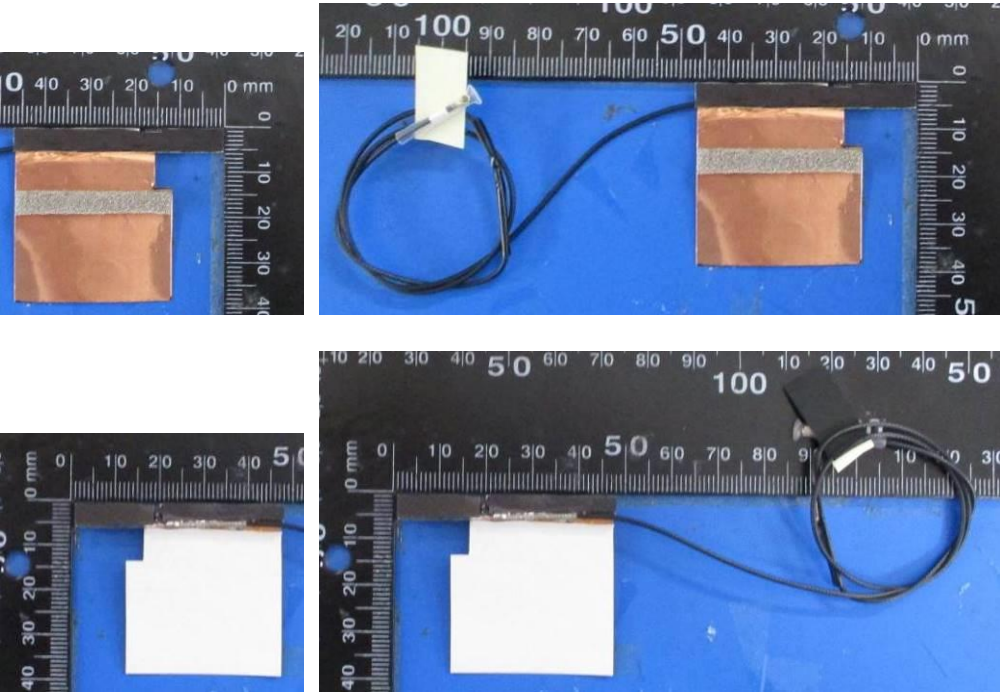
Tx1 Antenna Photo:
