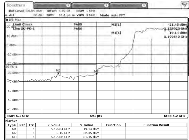
ax40-5190-PK-SISO A
