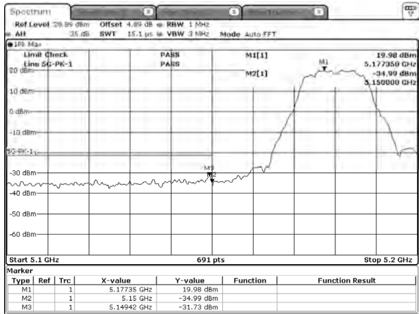
a-5180-SISO B-PK
