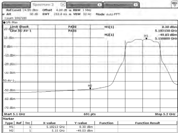
ax20-5180-SISO B-AV
