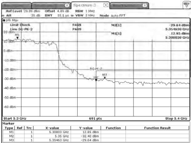
ax160-5250-996-S67-PK-SISO B-RU
