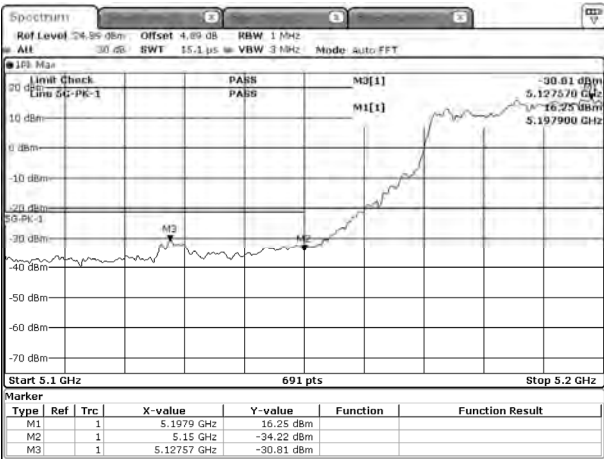
ax80-5210-PK-SISO A
