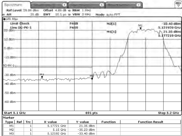
ax20-5180-SISO B-PK
