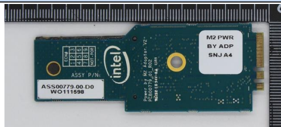
Socket back
