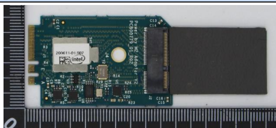
Socket front
