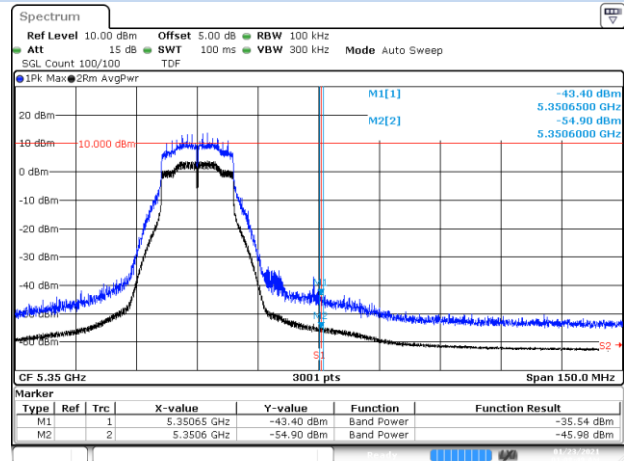
BE-R-HIGH, SISO-A, 802.11n20-HT0, Ch64
