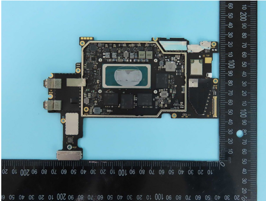
Figure 1: Main PCB with shields
