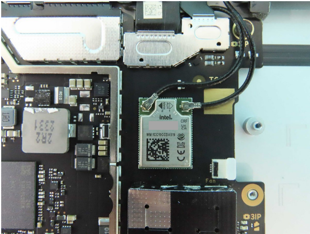
Figure 3: RF module
