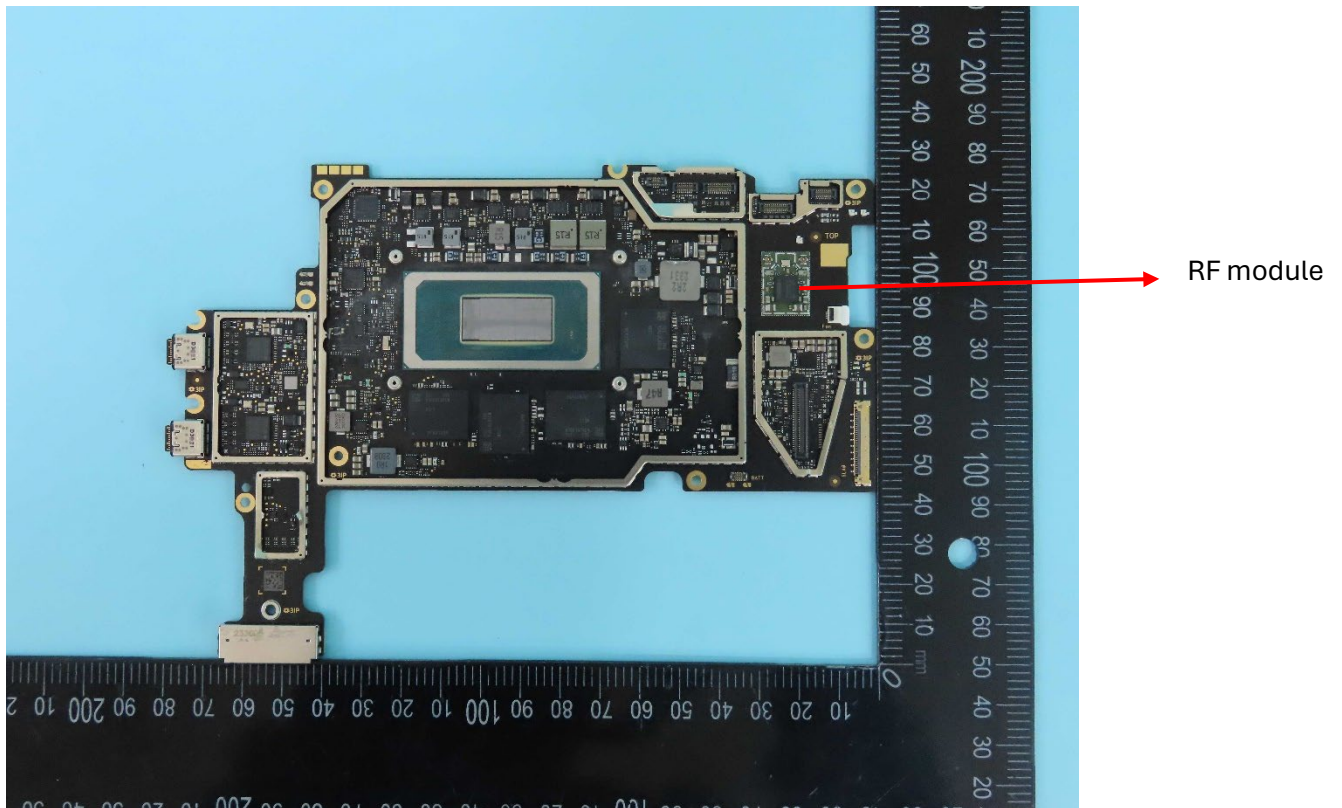
Figure 2: Main PCB with RF shield removed
