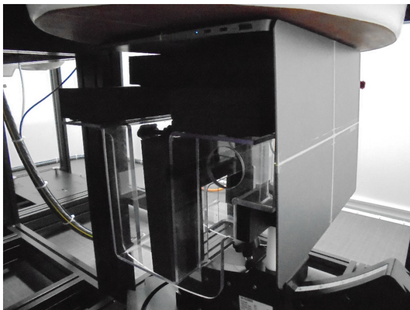
Bottom of EUT with 0mm Gap
