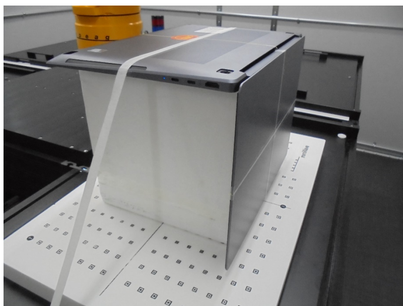
Bottom of EUT Power Density Setting
