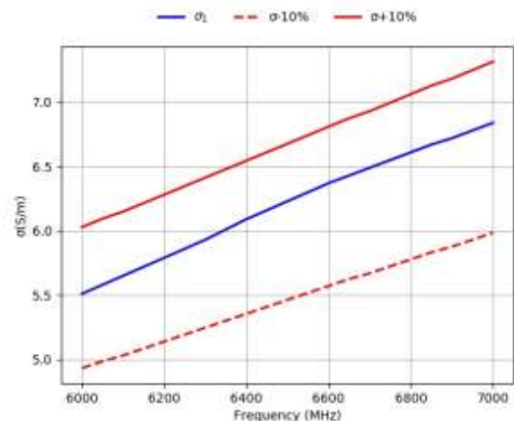
Conductivity
