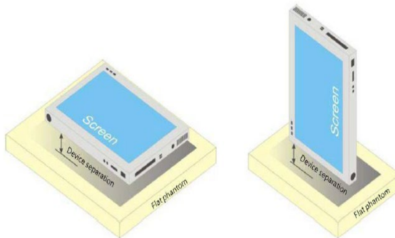
Fig-5.2 Illustration for Tablet Setup
