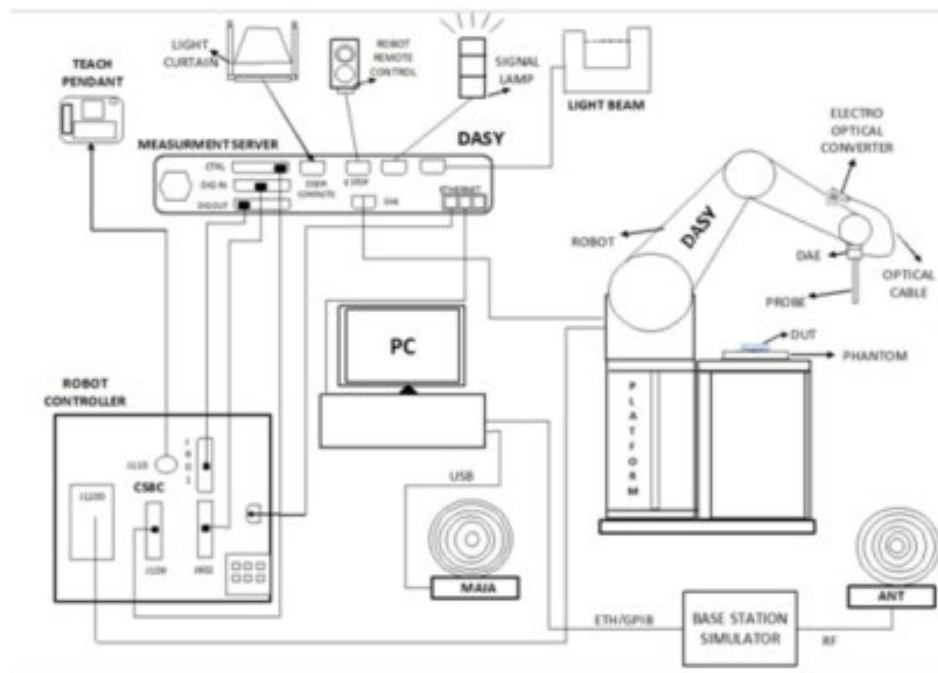
Fig-4.1 SPEAG DASY System Configuration
