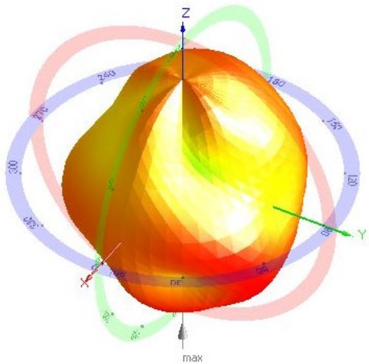
Max Antenna 3D Radiation Pattern 5150-5250 MHz
