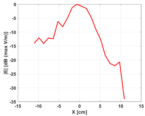
Field variation through the maximum along the H-field polarization
