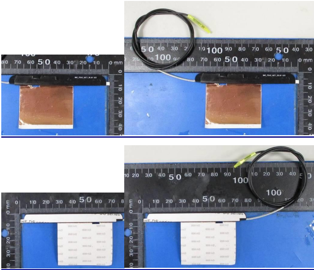
Main Antenna Photo (Front/Back):
