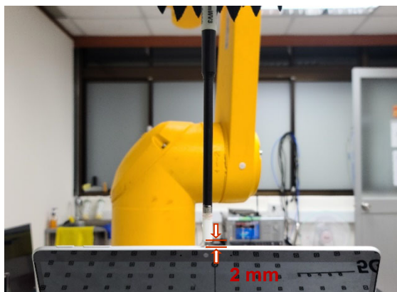
Photograph 15. PD, Top Tilt, 2mm
