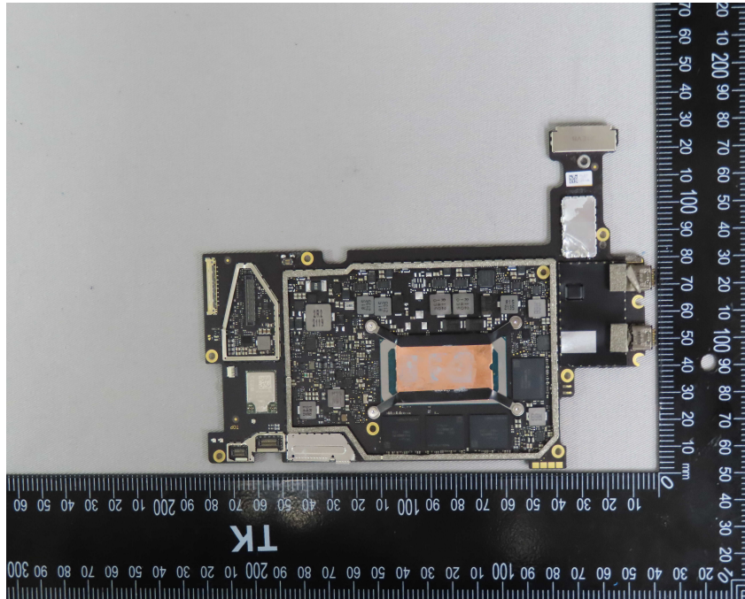
PCB top side
