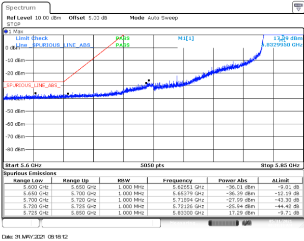
BE-NR-LOW, SISO-B, 802.11ac80-VHT0, Ch171
