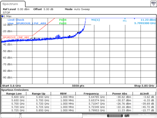
BE-NR-LOW, MIMO-A, 802.11ac160-VHT0, Ch163
