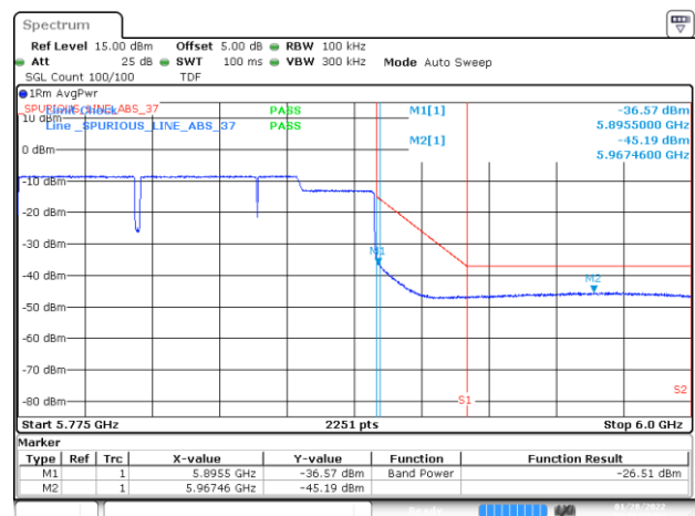
BE-NR-HIGH, SISO-B, 802.11ax160-HE0, Ch163
