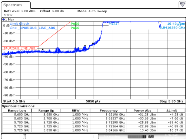
BE-NR-LOW, MIMO-B, 802.11ac160-VHT0, Ch163
