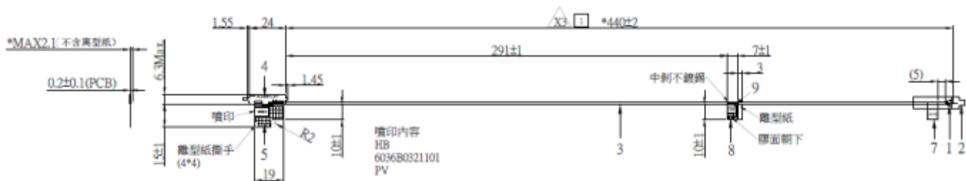
Tx1 Antenna Dimensioned Drawing:
