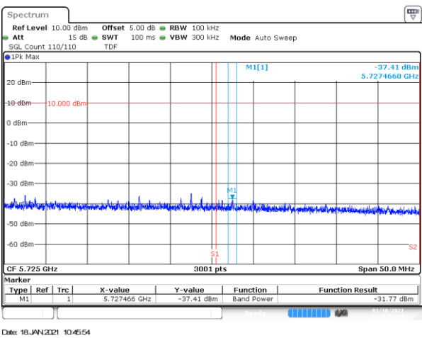
BE-NR-HIGH, MIMO-B, 802.11ax160-HE0, Ch114
