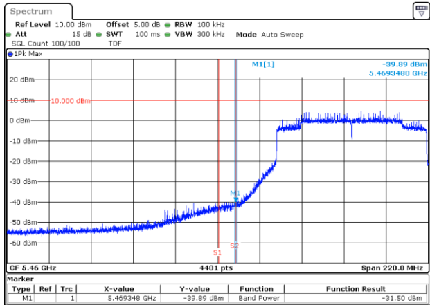
BE-NR-LOW, MIMO-A, 802.11ax80-HE0, Ch106
