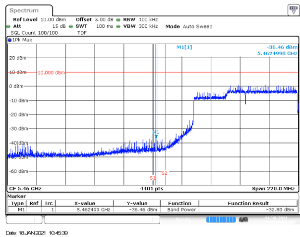
BE-NR-LOW, MIMO-B, 802.11ax160-HE0, Ch114
