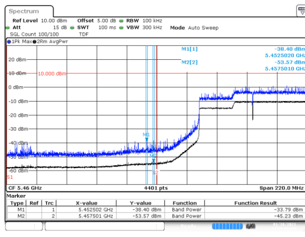
BE-R-LOW, MIMO-B, 802.11ax160-HE0, Ch114
