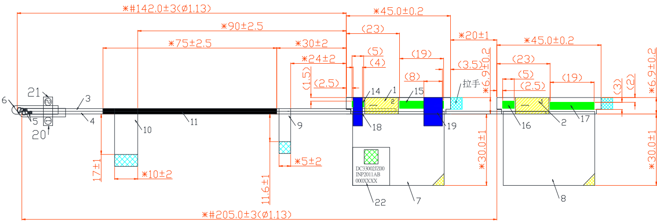
Tx1 Antenna Dimensioned Drawing:
