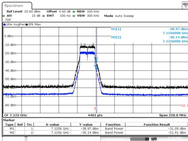
BE-NR-HIGH, MIMO-B, 802.11n20-HT8, Ch233
