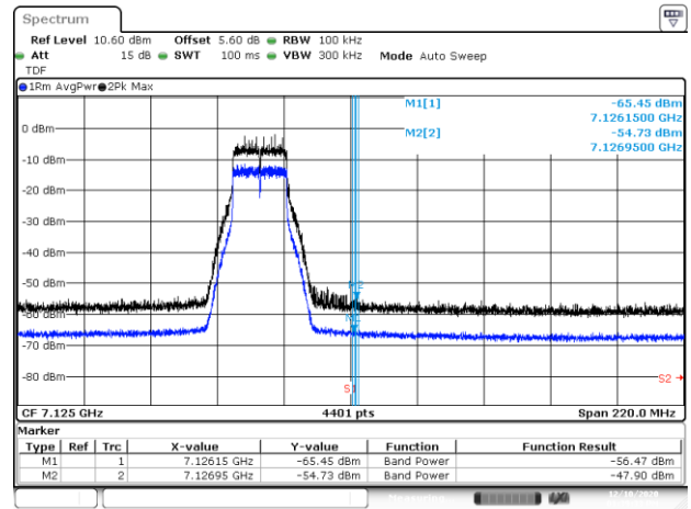
BE-NR-HIGH, MIMO-B, 802.11n20-HT8, Ch229
