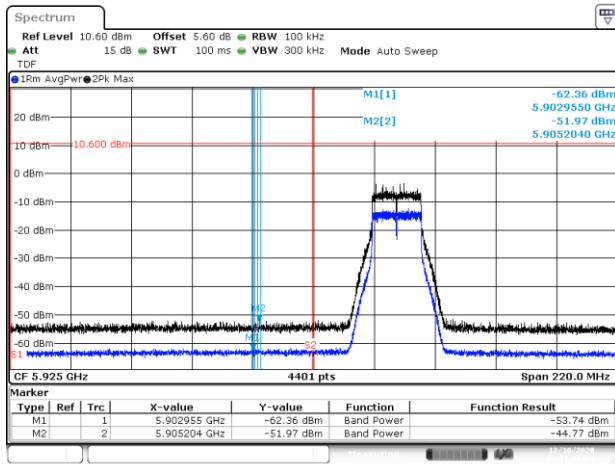
BE-NR-LOW, MIMO-B, 802.11n20-HT8, Ch1
