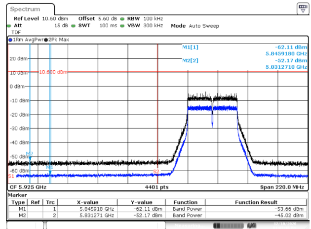
BE-NR-LOW, MIMO-B, 802.11n40-HT8, Ch3
