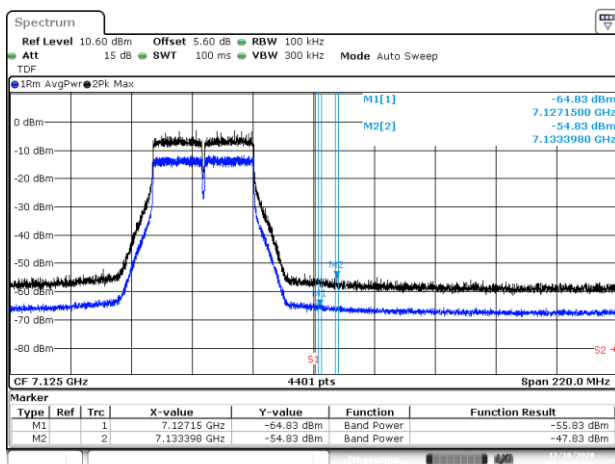
BE-NR-HIGH, MIMO-B, 802.11n40-HT8, Ch227
