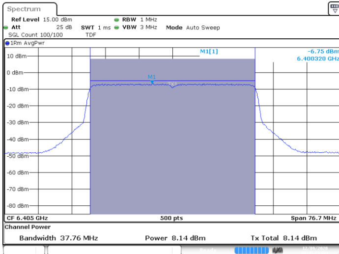
SISO A-802.11ax-40MHz-Ch91-6405MHz-HE0
