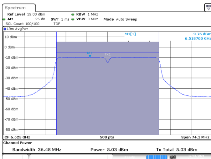
MIMO A-802.11n-40MHz-Ch115-6525MHz-HT8
