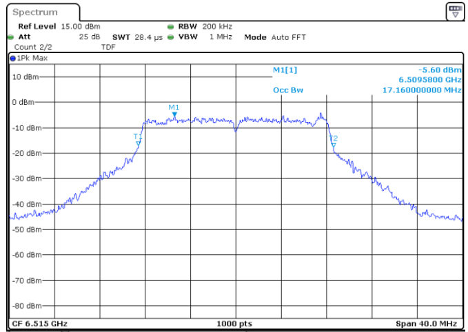
UNII6 SISO A 802.11a20 ch113 6515MHz 99%
