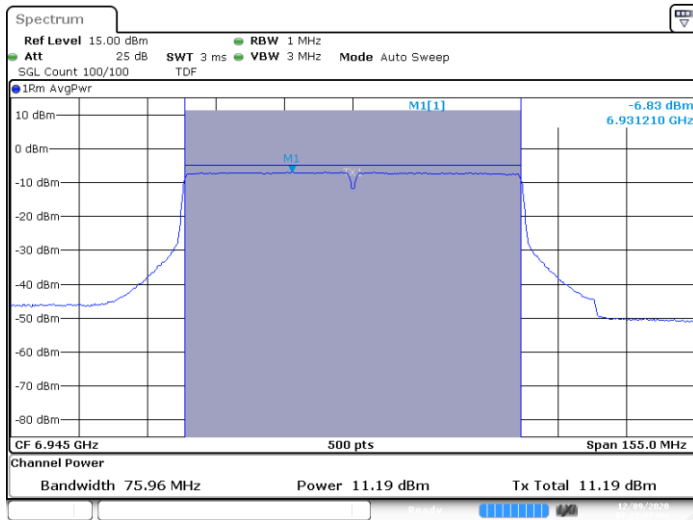
SISO A-802.11ac-80MHz-Ch199-6945MHz-VHT0
