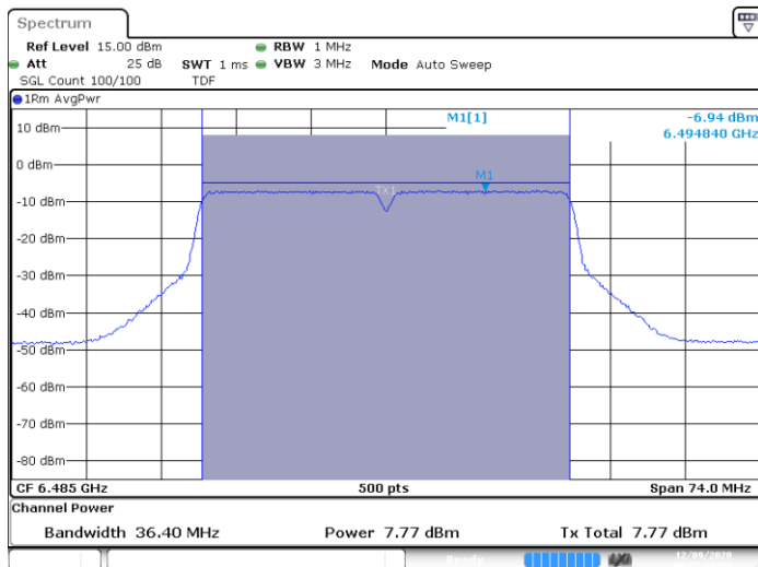
SISO A-802.11n-40MHz-Ch107-6485MHz-HT0
