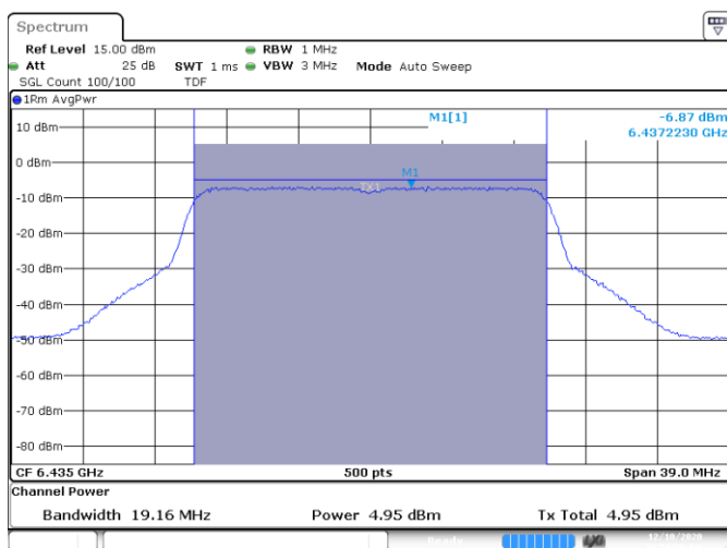
SISO B-802.11ax-20MHz-Ch97-6435MHz-HE0
