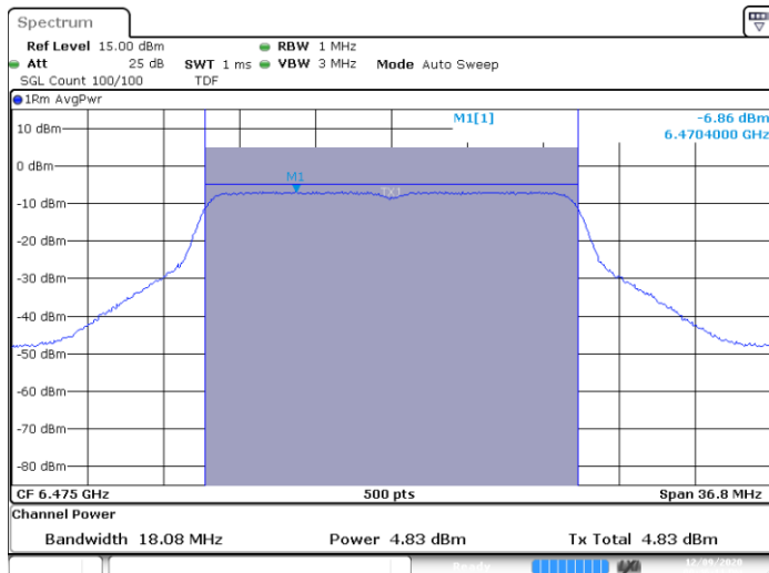
SISO A-802.11n-20MHz-Ch105-6475MHz-HT0
