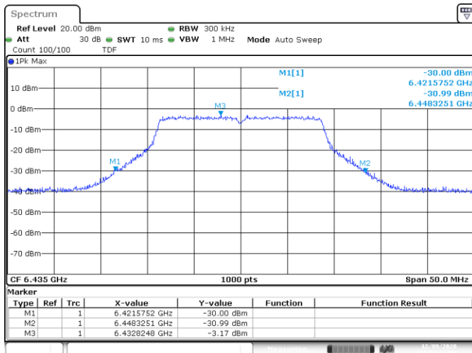
UNII6 SISO A 802.11n20 ch97 6435MHz 26dB
