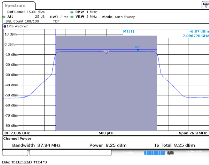
SISO B-802.11ax-40MHz-Ch227-7085MHz-HE0
