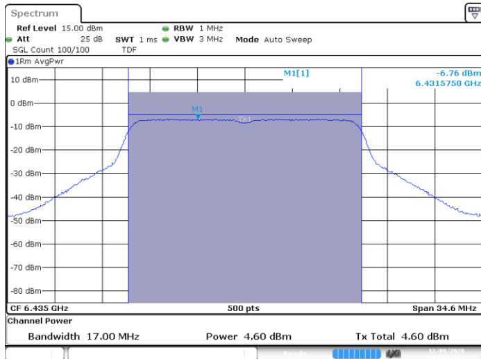
SISO A-802.11a-20MHz-Ch97-6435MHz-6
