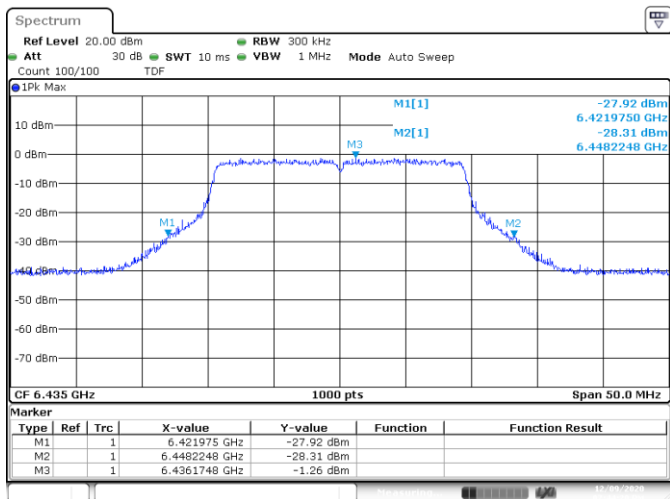
UNI16 SISO B 802.11ax20 ch97 6435MHz 26dB
