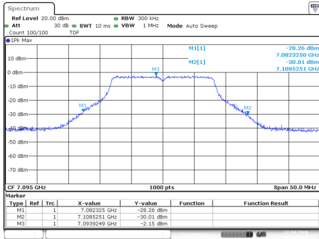
UNII8 SISO B 802.11a20 ch229 7095MHz 26dB
