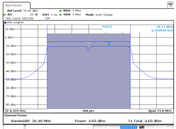
MIMO B-802.11n-40MHz-Ch115-6525MHz-HT8
