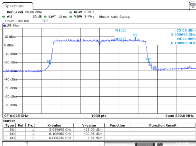
UNII5 SISO A 802.11ax160 ch15 6025MHz 26dB
