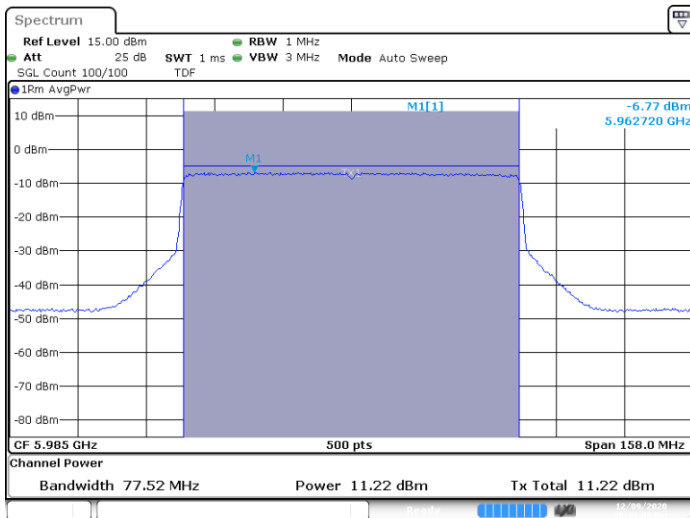
SISO A-802.11ax-80MHz-Ch7-5985MHz-HE0
