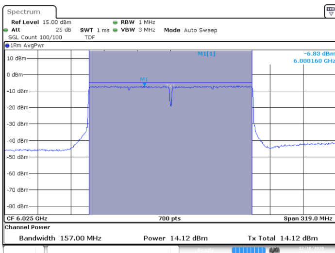
SISO A-802.11ax-160MHz-Ch15-6025MHz-HE0
