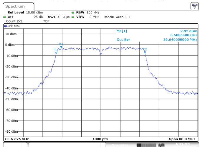
UNII7 SISO B 802.11n20 ch117 6535MHz 99%
