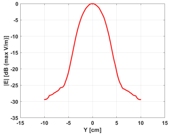
Field variation through the maximum along the E-field polarization
