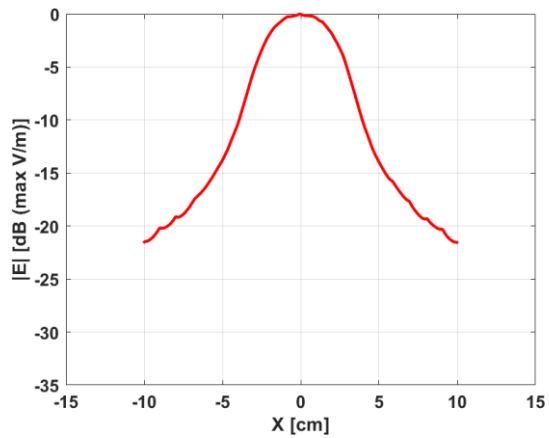
Field variation through the maximum along the H-field polarization
