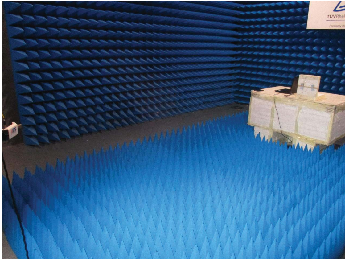
Photo 4: Photograph radiated emissions 26.5 – 36 GHz
