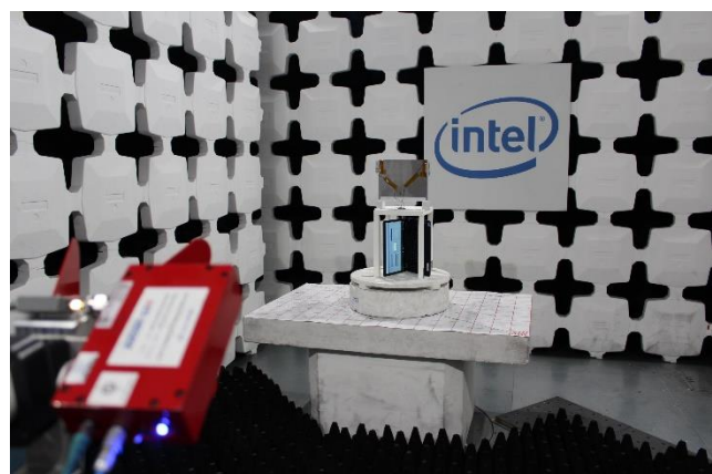
6.4 GHz – 18 GHz
