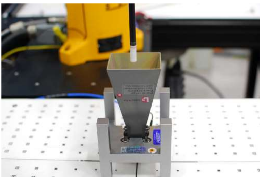
[Figure 3. System Verification Setup Photo]
