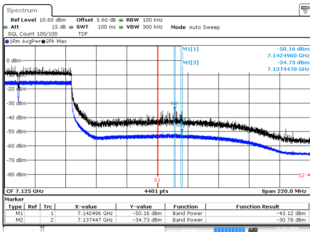
BE-NR-HIGH, MIMO-B, 802.11ac160-VHT0, Ch207
