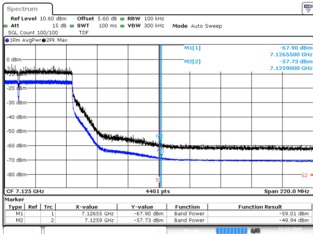
BE-NR-HIGH, MIMO-B, 802.11ac80-VHT0, Ch215
