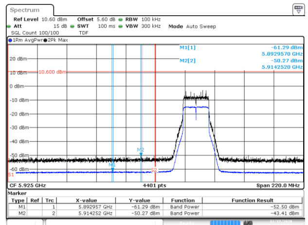
BE-NR-LOW, MIMO-B, 802.11ax20-HE0, Ch1
