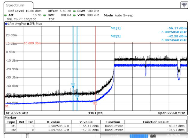
BE-NR-LOW, MIMO-B, 802.11ac160-VHT0, Ch15
