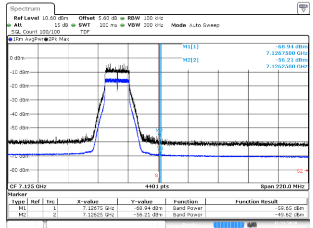
BE-NR-HIGH, MIMO-B, 802.11n20-HT0, Ch229
