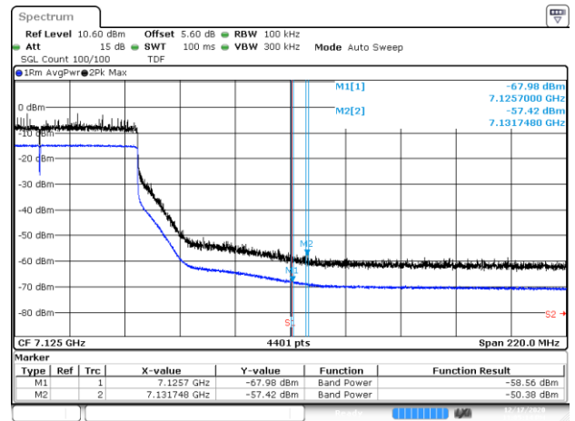
BE-NR-HIGH, MIMO-B, 802.11ac80-HE0, Ch215
