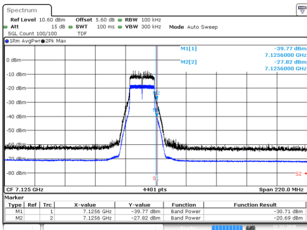
BE-NR-HIGH, MIMO-B, 802.11n20-HT0, Ch233
