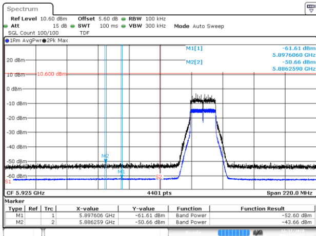
BE-NR-LOW, MIMO-B, 802.11n20-HT0, Ch1
