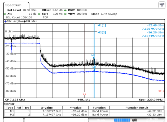
BE-NR-HIGH, MIMO-B, 802.11ac160-HE0, Ch207
