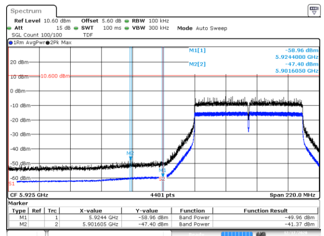
BE-NR-LOW, MIMO-B, 802.11ac80-VHT0, Ch7
