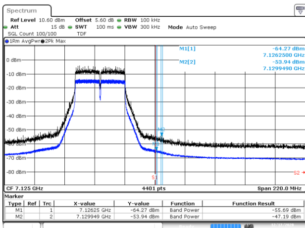
BE-NR-HIGH, MIMO-B, 802.11n40-HT0, Ch227
