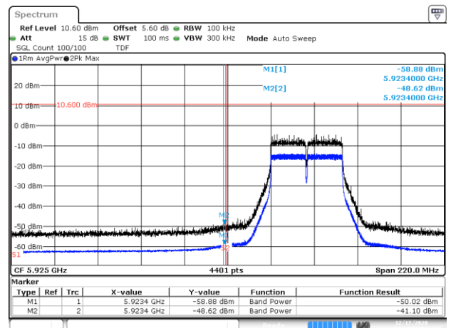
BE-NR-LOW, MIMO-B, 802.11n40-HT0, Ch3
