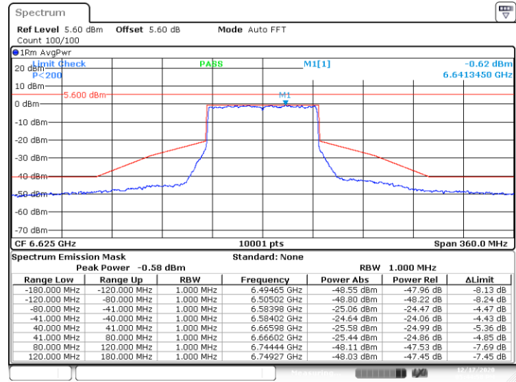
Channel 135
