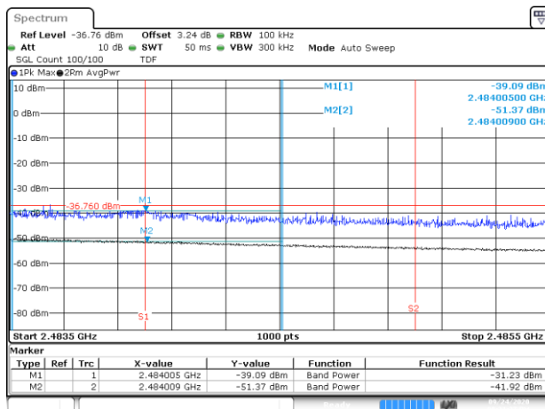
BE-R-HIGH-2MHz, SISO-A, 802.11ax40-HE0, Ch12
