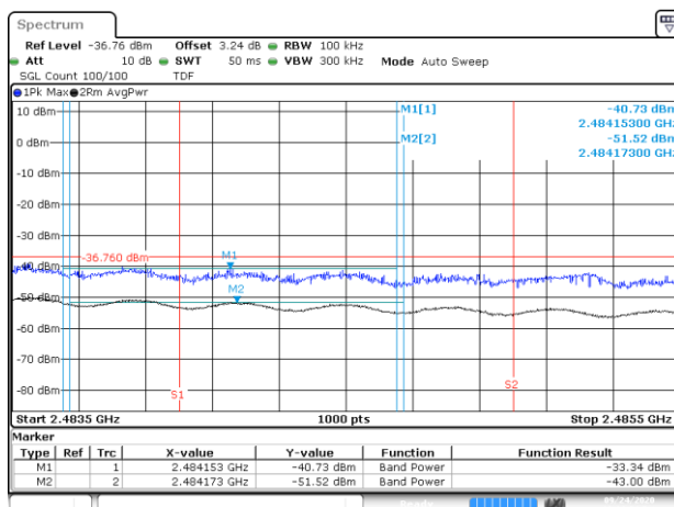
BE-R-HIGH-2MHz, SISO-A, 802.11n40-HT0, Ch12
