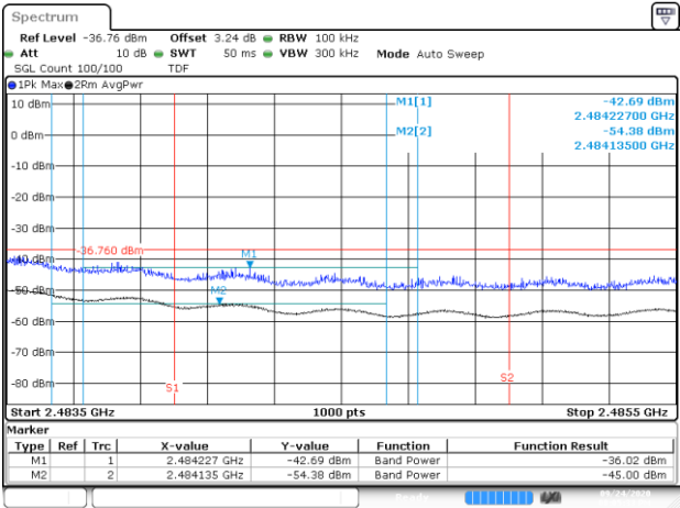
BE-R-HIGH-2MHz, SISO-A, 802.11n40-HT0, Ch13
