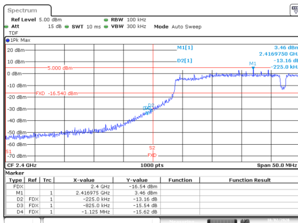
BE-NR, SISO-A, 802.11n40-HT0, Ch1
