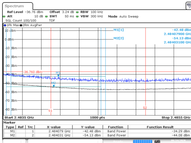
BE-R-HIGH-2MHz, SISO-A, 802.11ax40-HE0, Ch13
