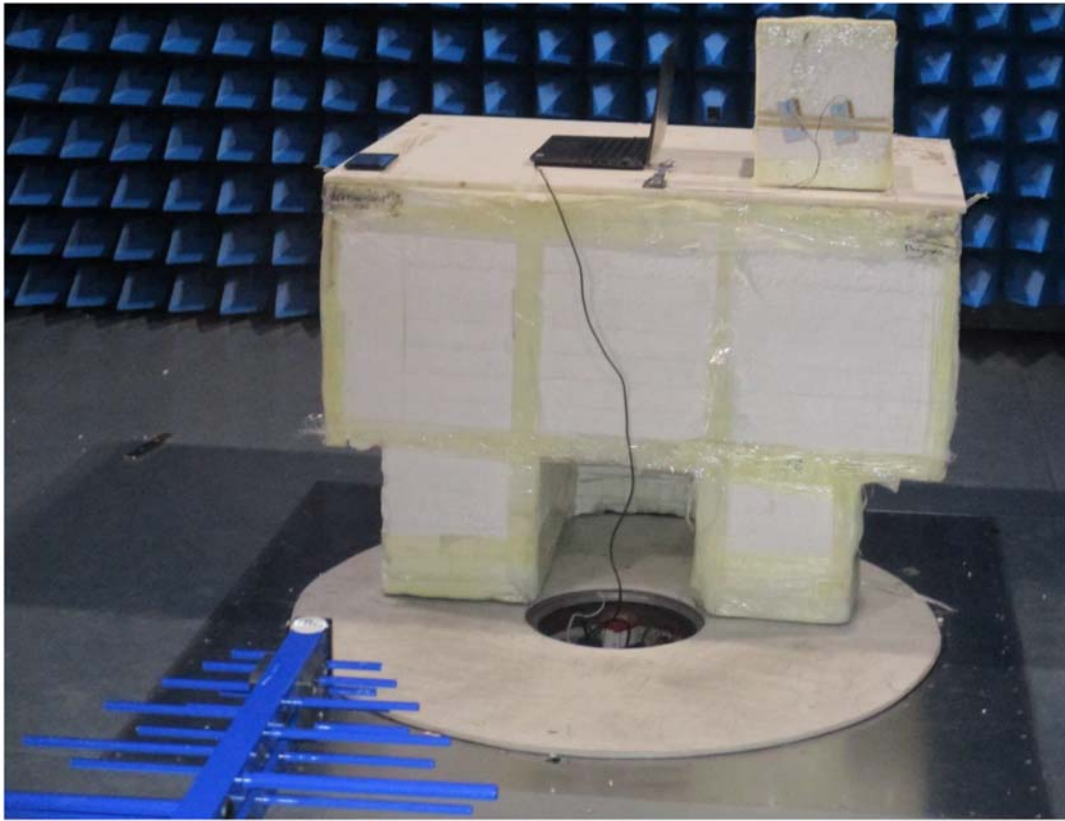
Photo 1 Photograph test setup radiated emissions 30-1000 MHz
