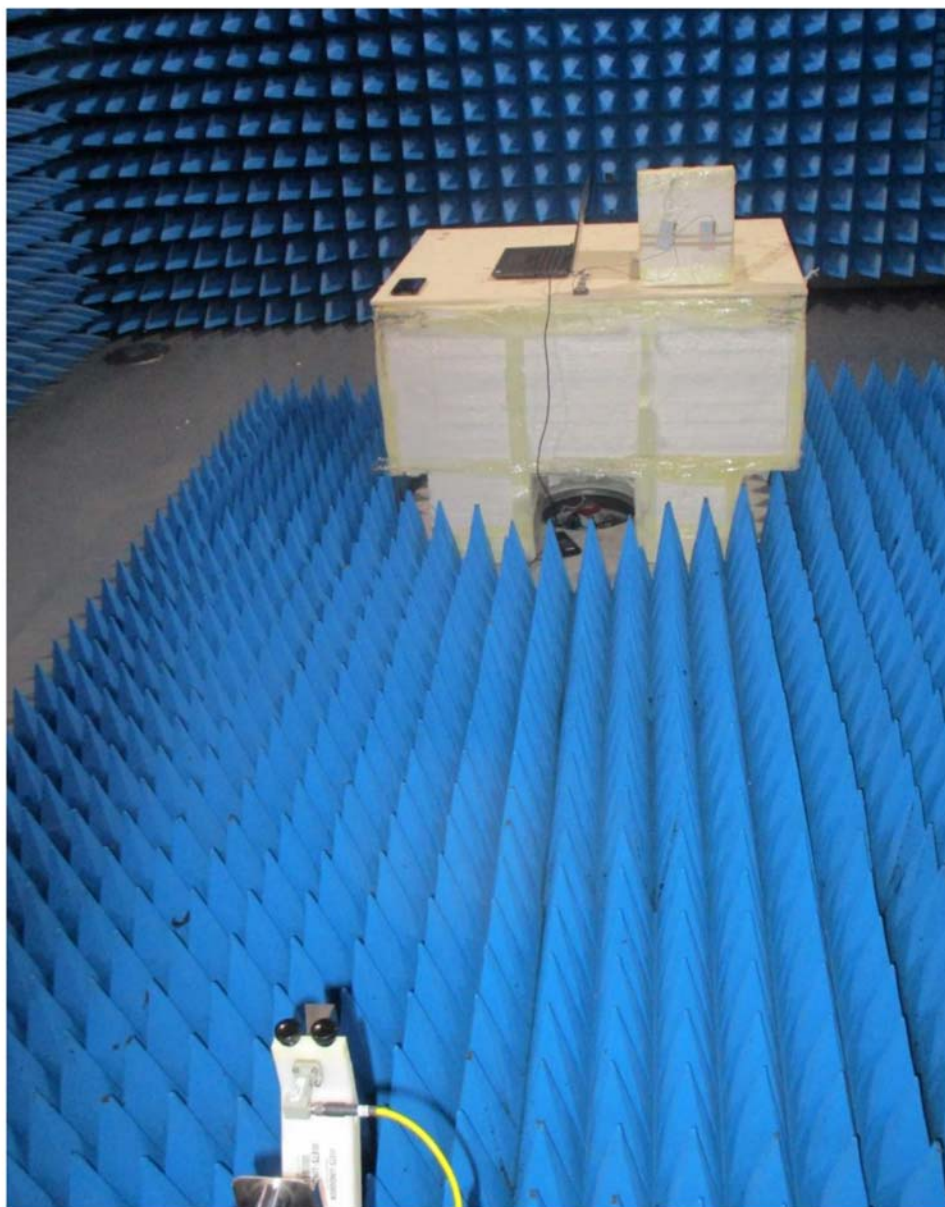
Photo 4: Photograph radiated emissions 26.5 – 36 GHz
