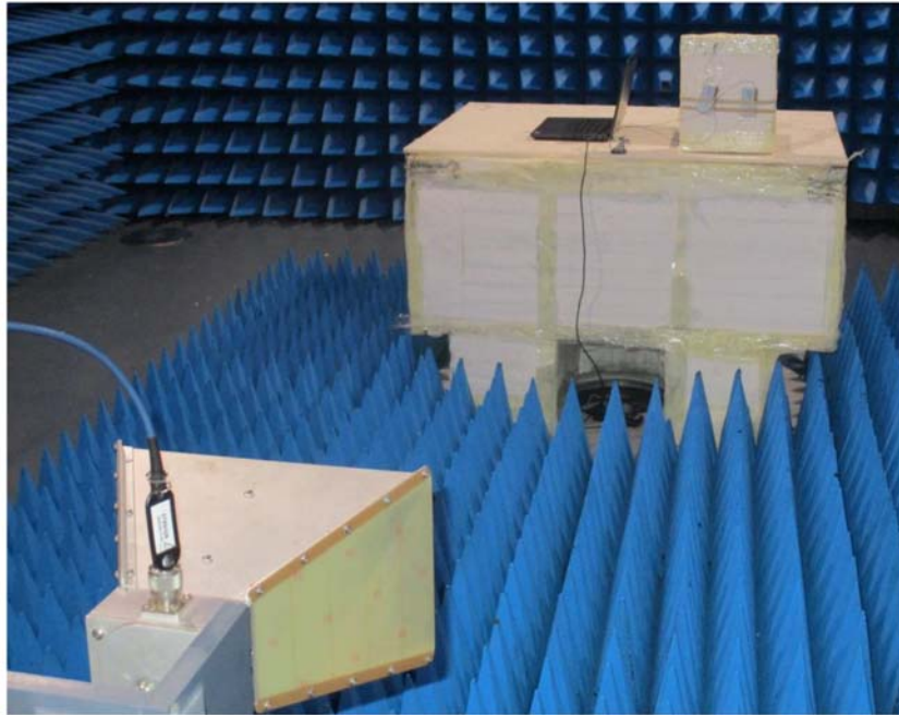
Photo 2: Photograph radiated emissions 1 – 18 GHz
