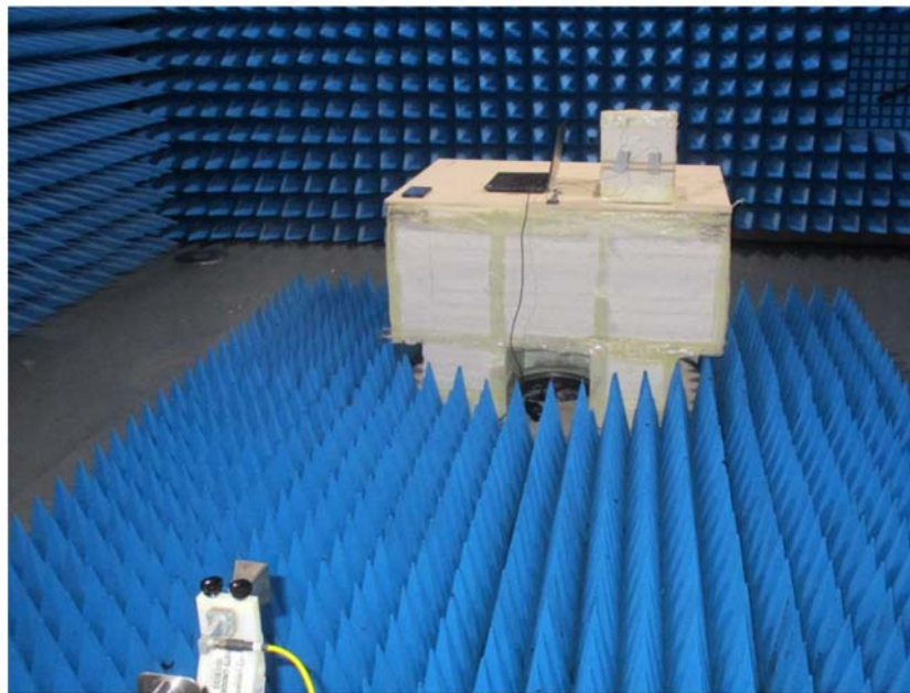
Photo 3: Photograph radiated emissions 18 – 26.5 GHz
