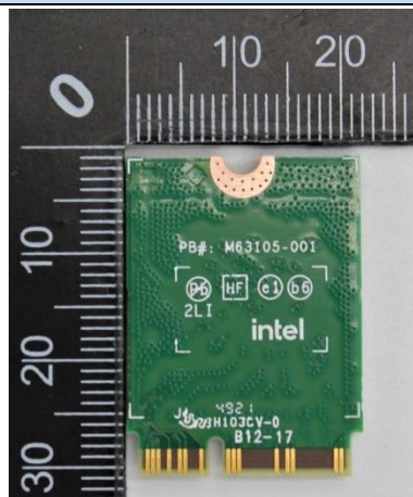
Adaptor back
