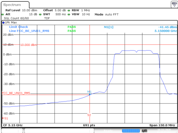
BE-R-LOW-Peak-10Hz, SISO-A, 802.11ax40-HE0, Ch38
