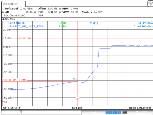
BE-R-LOW-Peak-10Hz, SISO-A, 802.11ax80-HE0, Ch42
