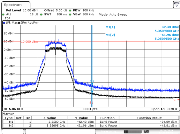
BE-R-HIGH, SISO-A, 802.11n20-HT0, Ch64
