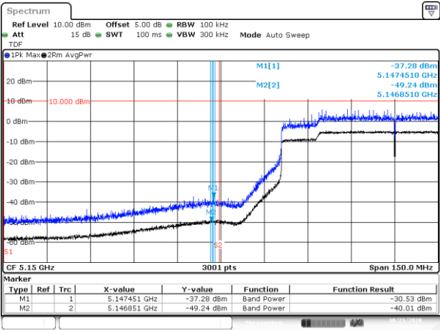
BE-R-LOW, SISO-A, 802.11ax80-HE0, Ch42-Only Peak
