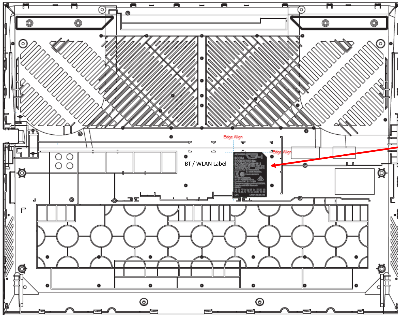
Galio16 Label Plan Bottom Core Side Label
