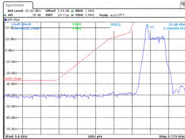
Peak (Partial RU: 26/0)
