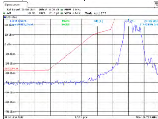
Peak (Partial RU: 106/53)
