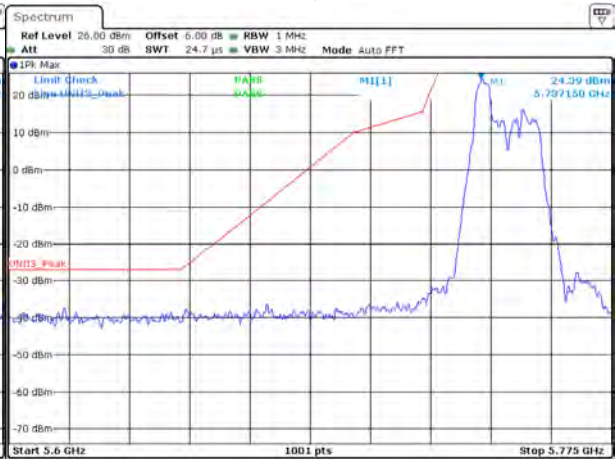
Peak (Partial RU: 52/37)
