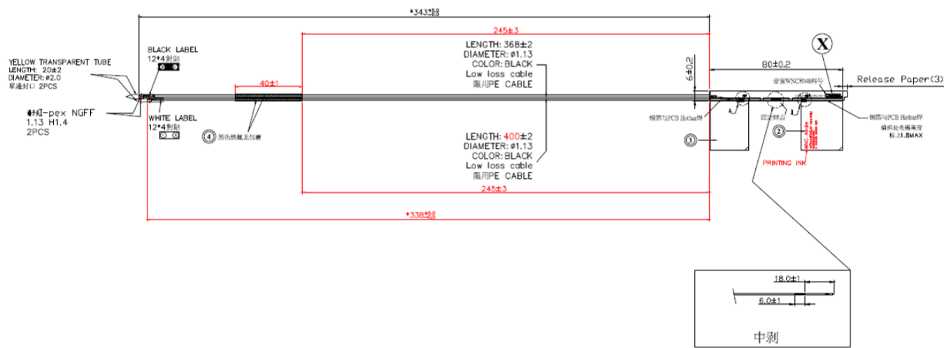
Tx1 (AUX) Antenna Dimensioned Drawing:
