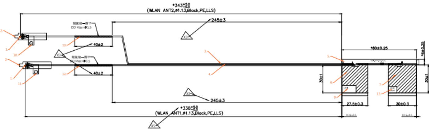
Tx1 (AUX) Antenna Dimensioned Drawing:
