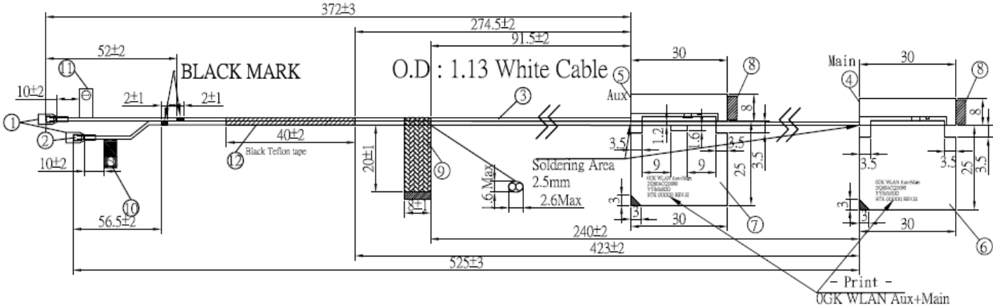
Tx1 Antenna Dimensioned Drawing:
